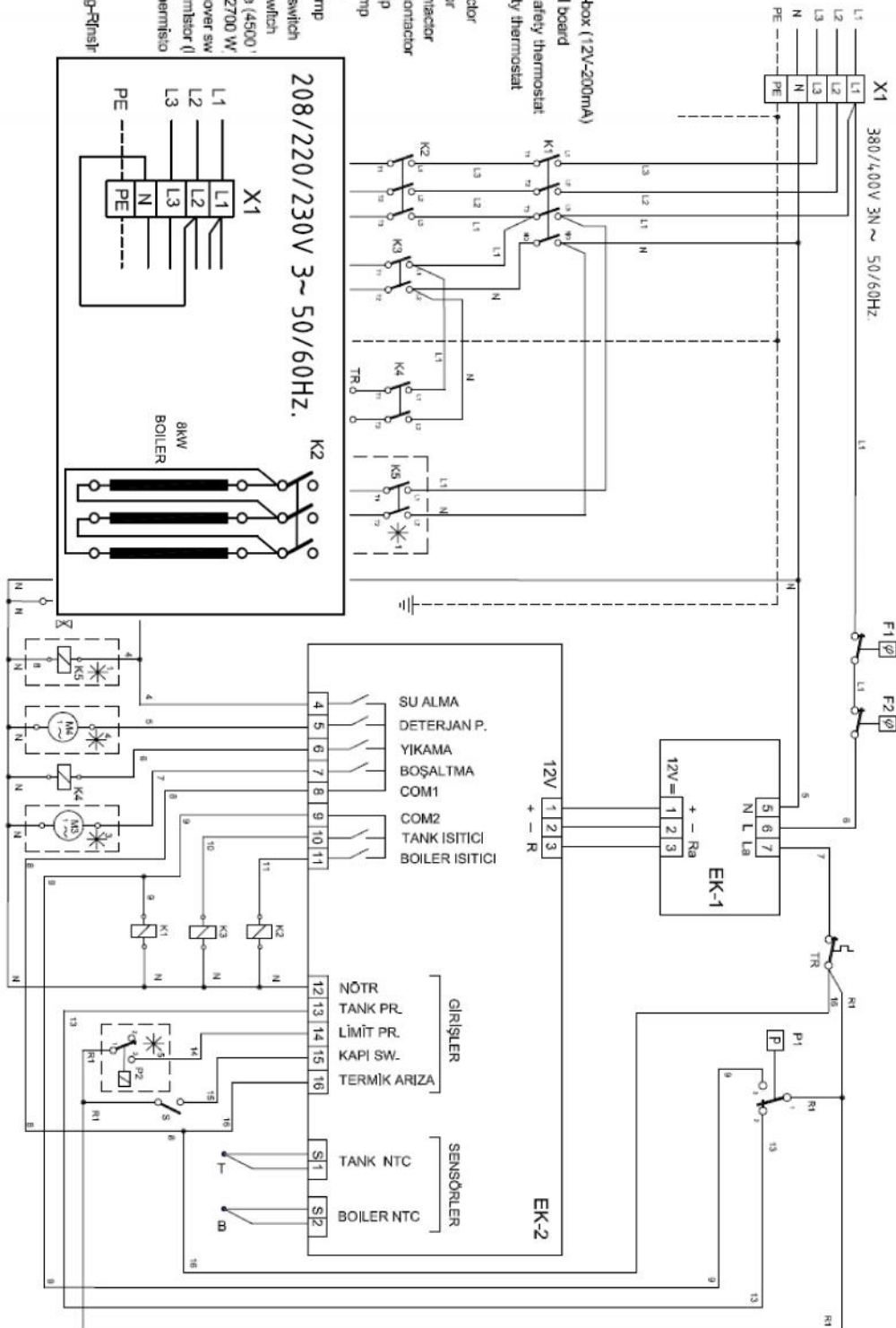
BYM 102 ELECTRIC SCHEMA
